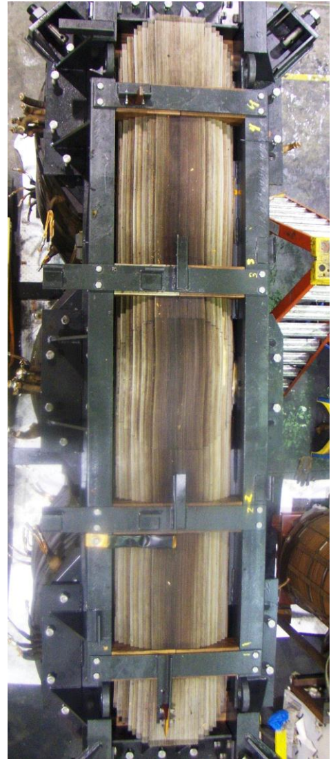
Overhead view of top yolk of core
