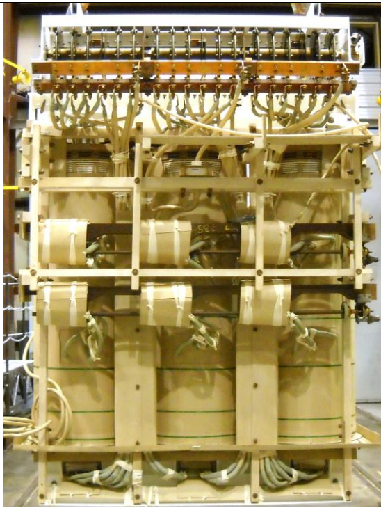
New leads & lead structure
