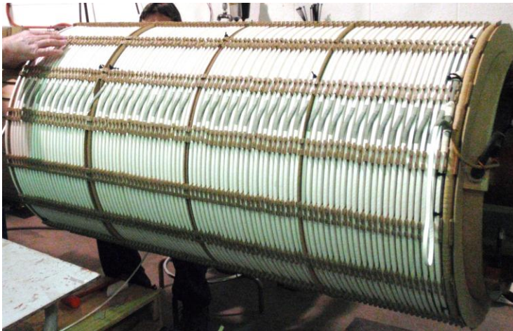
New copper windings with Nomex Insulation
