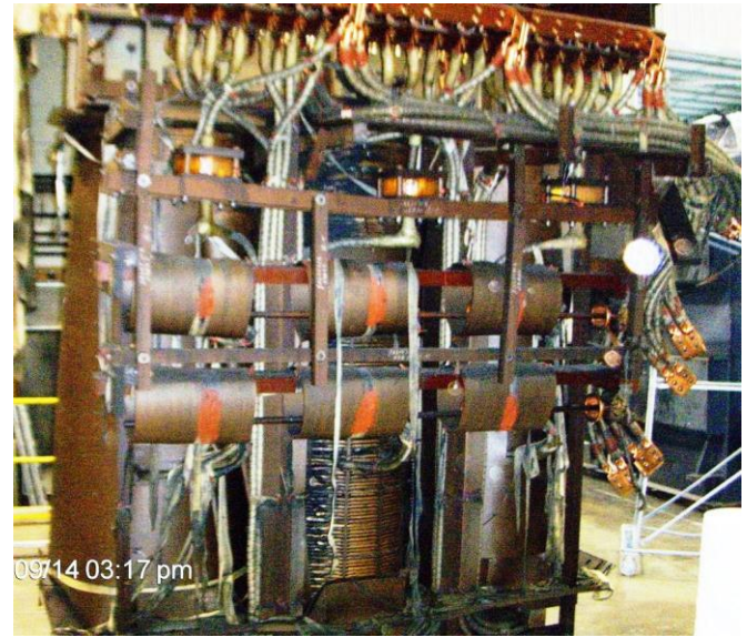
Core and Coil Assembly with Broken Lead Structure
