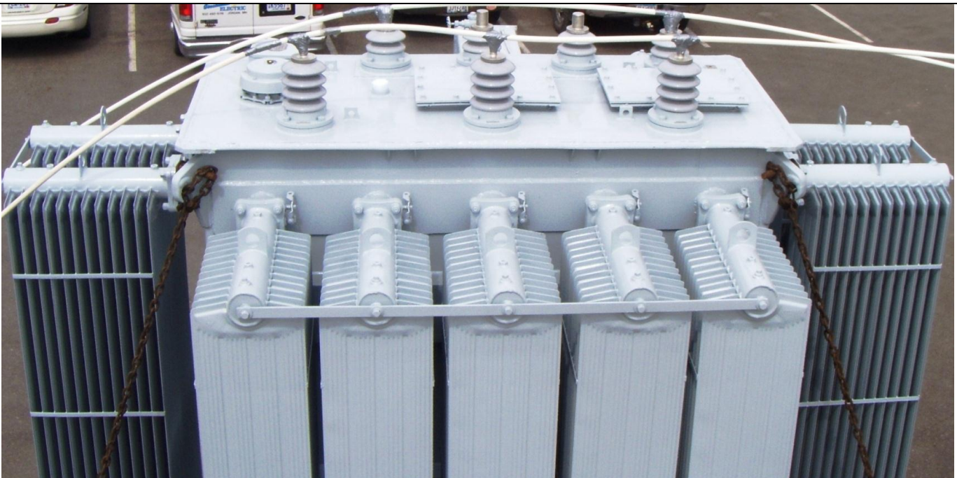
10/11.2 MVA OA @ 55/65° 13800 – 4160Y
