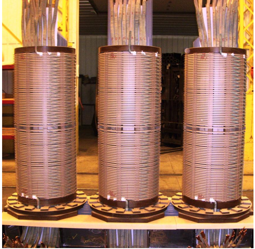
New Circular Disc Windings
